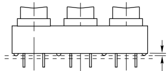
CIRCUIT BOARD STANDOFF .062 ± .010 - .005 (1,57 ± 0,25 - 0,13) DIA. x .032 ± .005 (0,81 ± 0,13) HIGH
